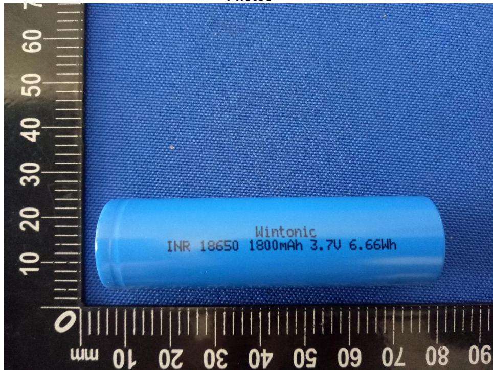
Fig.1 Front view of Battery
